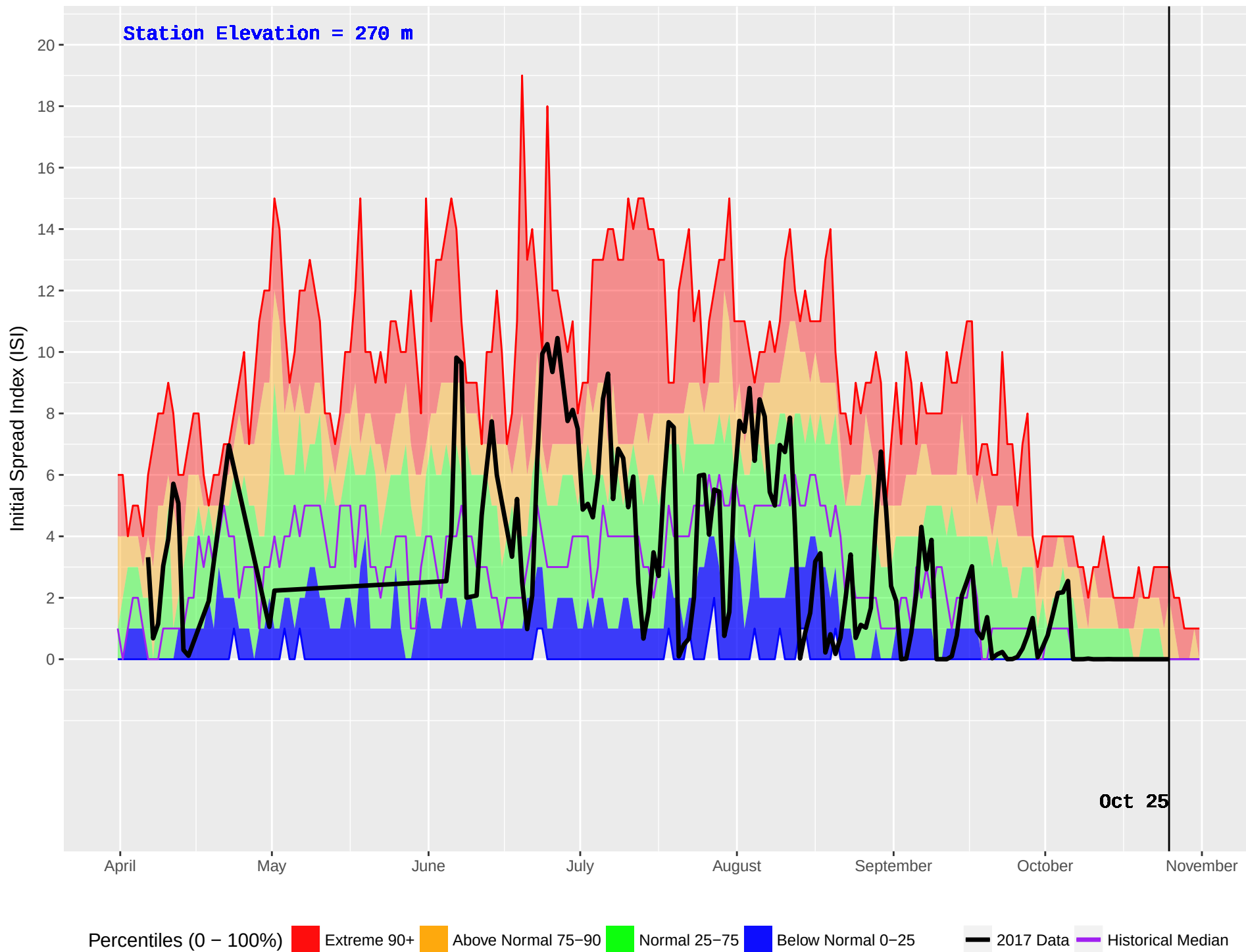
TALCHAKO (233) : Historical (1990–2016) and Current (2017) Noon Initial Spread Index (ISI)
