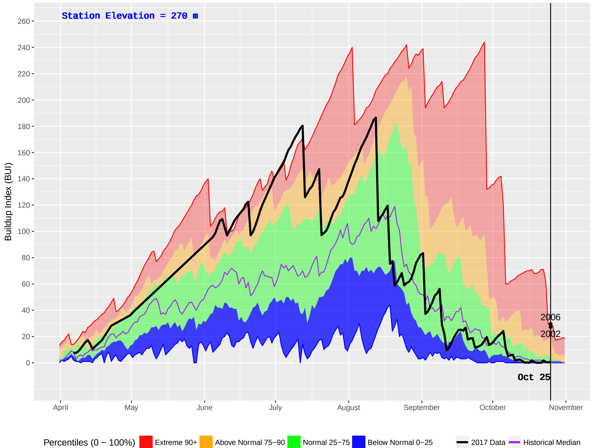
TALCHAKO (233) : Historical (1990–2016) and Current (2017) Noon Buildup Index (BUI)
