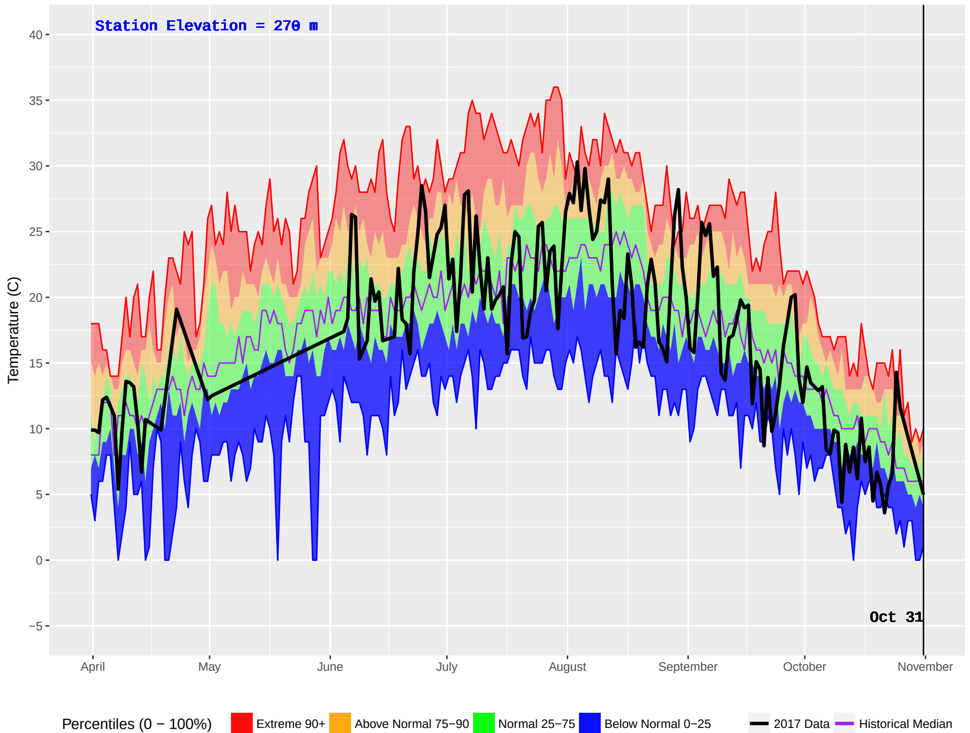
TALCHAKO (233) : Historical (1990–2016) and Current (2017) Noon Temperature
