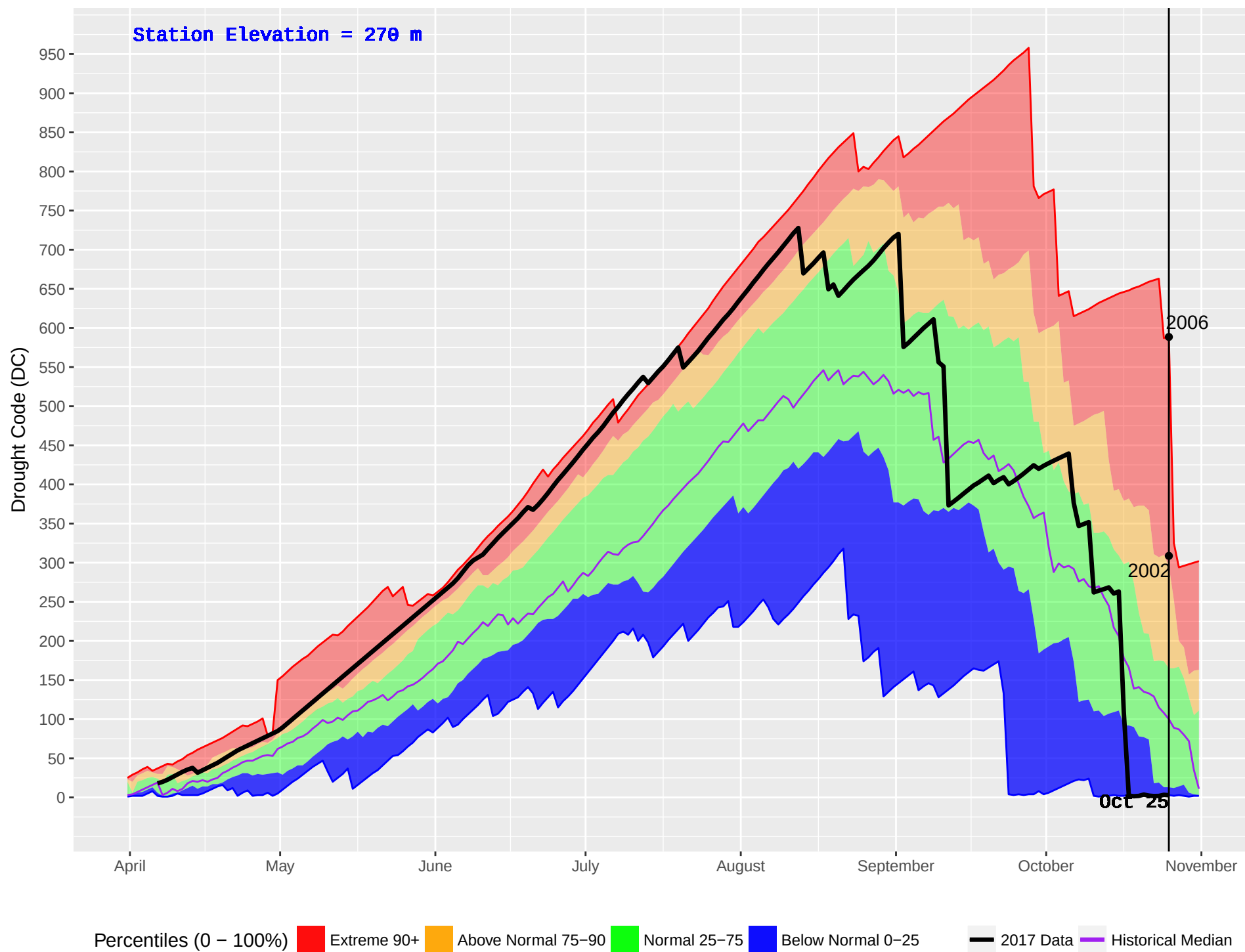
TALCHAKO (233) : Historical (1990–2016) and Current (2017) Noon Drought Code (DC)
