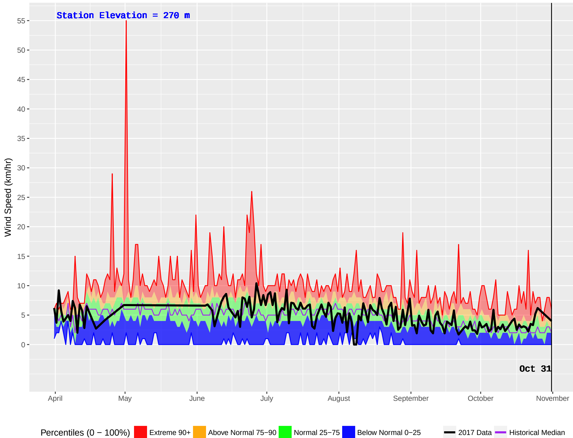
TALCHAKO (233) : Historical (1990–2016) and Current (2017) Noon Wind Speed
